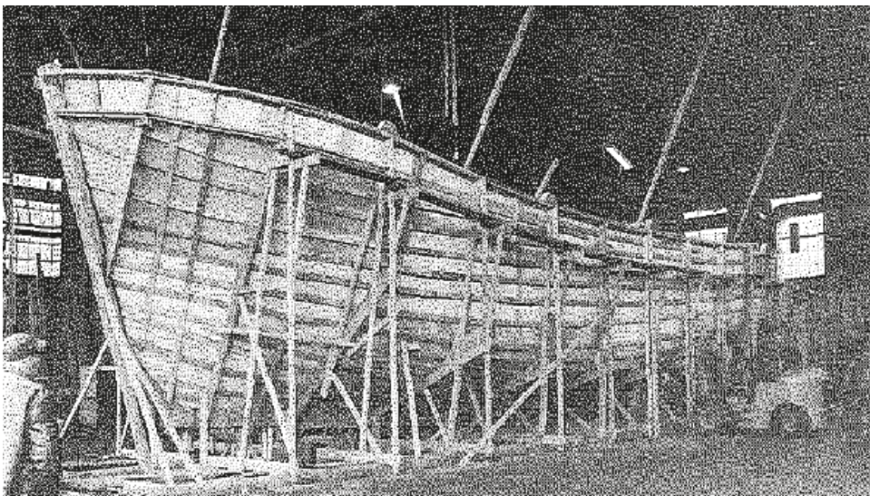
Exterior view of 58' split type mold developed by Shearwater Marine in 1969. Believed to be the largest mold of its type in Canada.
